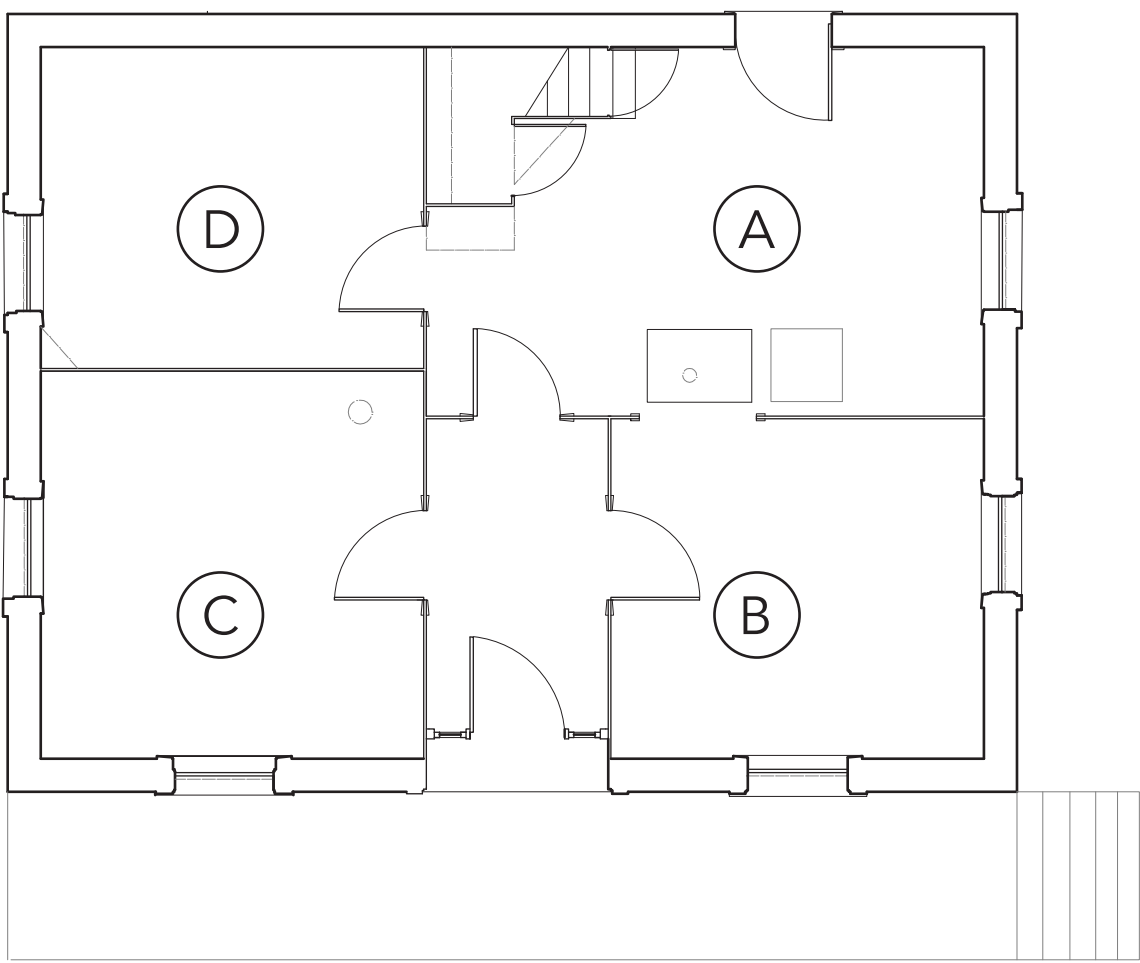
PLAN RDC - INITIAL / FIRST FLOOR PLAN - INITIAL
